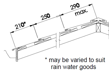
Figure 7.4 Lap Section
