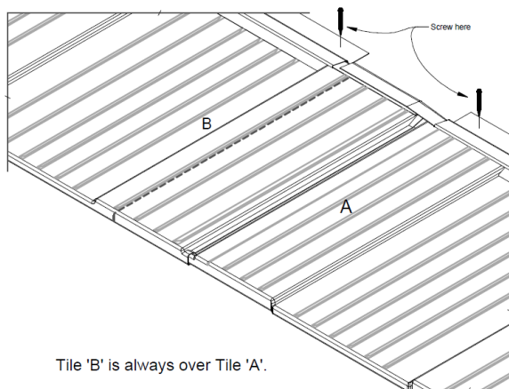
Figure 7.4 Lap Section
